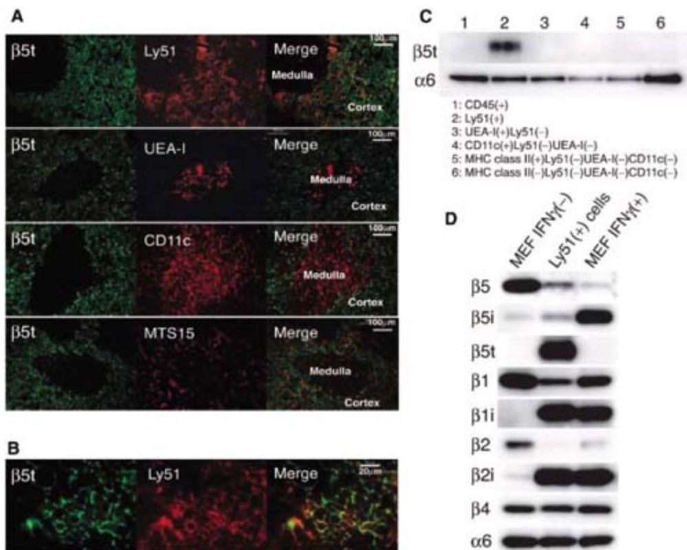
Fig. 3. \beta 5t is specifically expressed in cTECs. (A and B) Cryosections of mouse thymus were immunostained for \beta 5t , together with Ly51, UEA-I, CD11c, or MTS15. (C) Various populations of cells from the thymus were immunoblotted for \beta 5t and \alpha 6 (a loading control for proteasomes). (D) Contents of thymoproteasomes in Ly51-positive cells were analyzed by immunoblotting. MEF, murine embryonic fibroblast.
